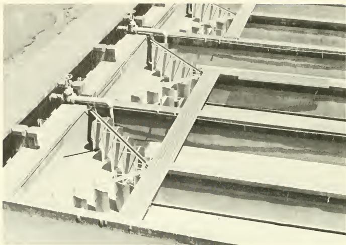
FIGURE 20. Rectangular circulation rearing pond ("Burrows pond"). Water is recirculated around the pond with the aid of turning vanes (arrow). Waste water flows out through floor drains located in the center wall (not shown). (FWS photo.)
