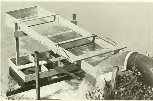
FIGURE 38. Box-type filters mounted in fixed positions. (Diagram from Arkansas Game and Fish Commission; photo courtesy of Fish Farming Experimental Station, Stuttgart, Arkansas.)
