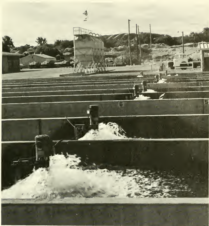
FIGURE 3. Electric powered aerators midway in a series of raceways can provide up to 2 ppm more oxygen for increased fish production. This type aerator is operated by a 1 horsepower motor and sprays approximately 1 cubic foot per second of water. Note the bulk storage bins for fish food in the center background. (Courtesy California Department of Fish and Game.)
