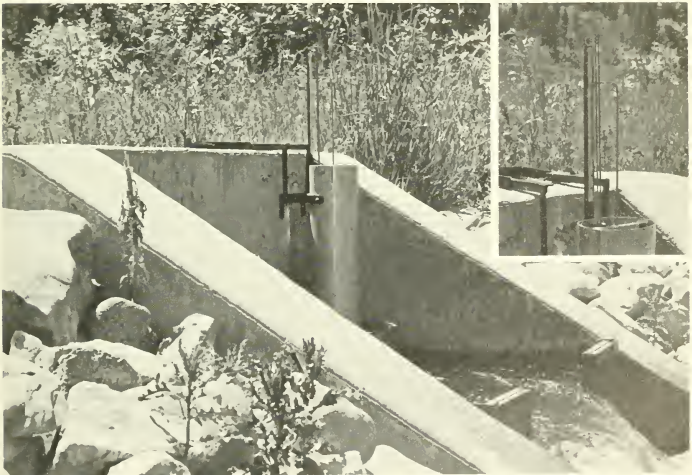
FIGURE D-1. (Top) Diagram of a Cippoletti weir plate. It should be cut from No. 8 or No. 10 galvanized iron plate. The trapezoidal notch must be cut to the exact dimensions as shown. Flow rates with this weir will be twice the values shown in Table D-1. (Bottom) A rectangular weir installed to measure water flow at the discharge of a fish hatchery. A sight gauge (insert) with a float in an aluminum cylinder is used to measure water depth over the crest of the weir. It must be positioned at a distance at least 2.5 times the depth of the water flowing over the weir.
