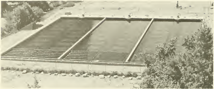
FIGURE 13. Three linear clarifiers located at the Jones Hole National Fish Hatchery, 114 ft \times 41 ft and 6 ft deep. Each unit has a sludge scraper system for sludge removal. These are long redwood boards attached by chain to move and deposit sludge into the sumps at the upper ends of the clarifiers. This system is designed to pump sludge to drying chambers. (FWS photo.)
