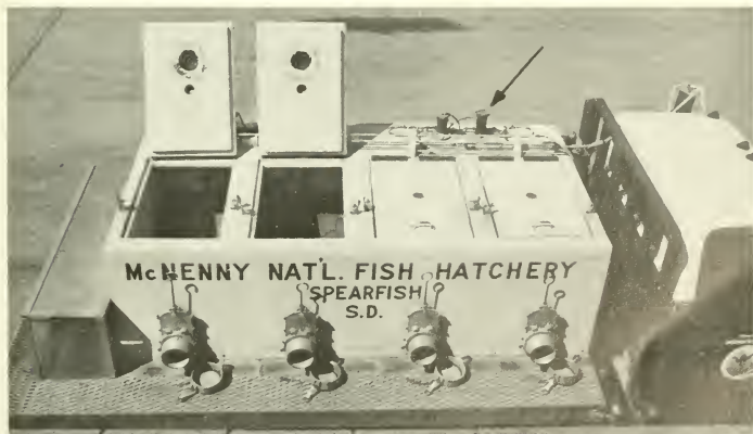
FIGURE 109. Fiberglass distribution tank with four compartments, each with an electric aerator (arrow). Additional oxygen is provided through carbon rods or micropore tubing on the bottom of the tank. (McNenny National Fish Hatchery, FWS.)
