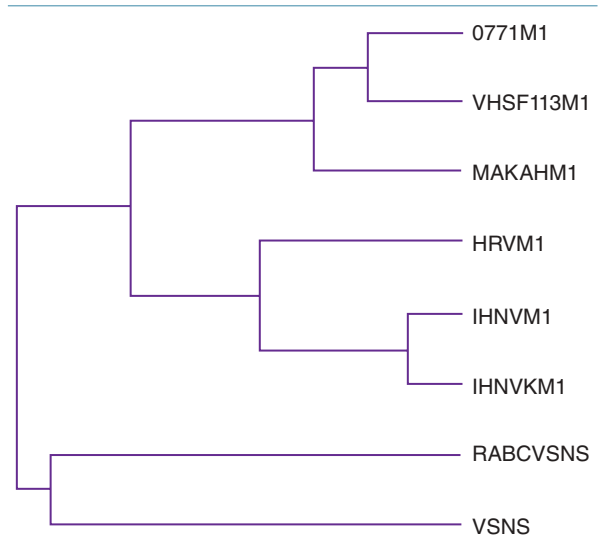
Figure 6.52 Dendrogram produced by CLUSTAL analyses of the deduced amino acid sequences of the M1 genes of HIRRV (HRVM1); two strains of IHNV, from North America (IHNVM1) and Europe (IHNVKM1); and three strains of VHSV, from Europe (0771M1, VHSF113M1) and North America (MAKAHM1). The amino acid sequence of the NS protein (equivalent to phosphoprotein or M1 protein) of rabies virus strain CVS (RABCVSNS) and vesicular stomatitis virus serotype New Jersey (VSVNS) were used as representatives of the lyssavirus and vesiculovirus genera, respectively. Nearly identical dendrograms were generated by comparison of the partial N and complete M2 amino acid sequences. (By courtesy of Inter-Research and Dr J.R. Winton.)
